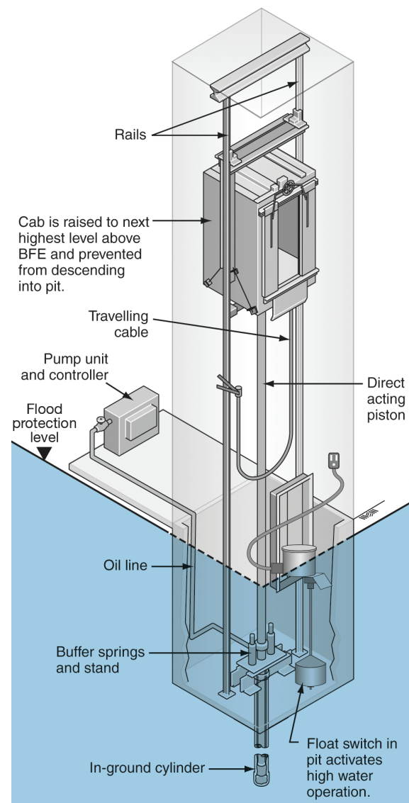
Figure 5-27. Float switch to control cab descent (Source: Otis Elevator Company).
